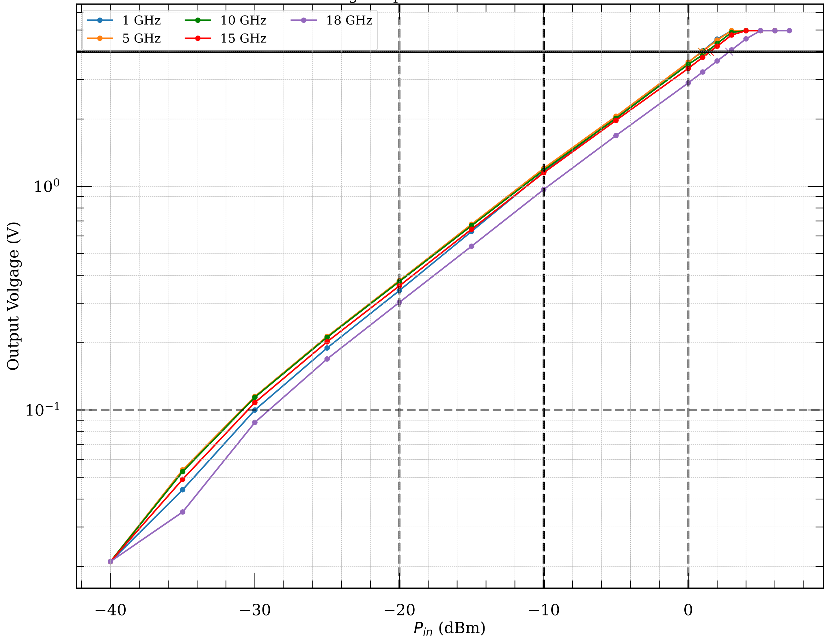
Measured voltage-to-power curve of detector module072
